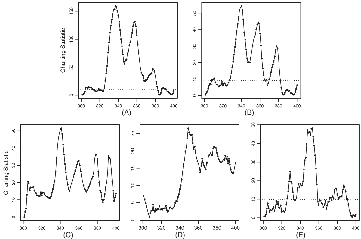
FIGURE 6 Control charts SS-MEWMA (plot (a)), SR-MEWMA (plot (b)), SR-CPD (plot (c)), XQ-CUSUM (plot (d)) and NEW (plot (e)) for monitoring the last 100 process observations shown in Figure 5. In each plot, the horizontal dotted line denotes the control limit of the related control chart
